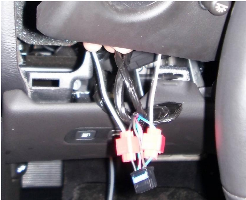
Figure 11. Use the provided wire taps to create power and ground wires for the gauge
